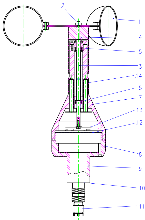
Fig. 1: Mechanical design
